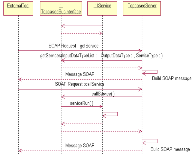
Figure 3: Communication from an external tool to TOPCASED.
