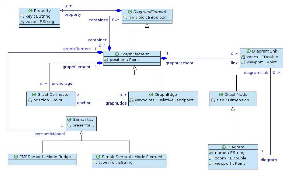
Figure 8: A simplified view of the XMI-DI
