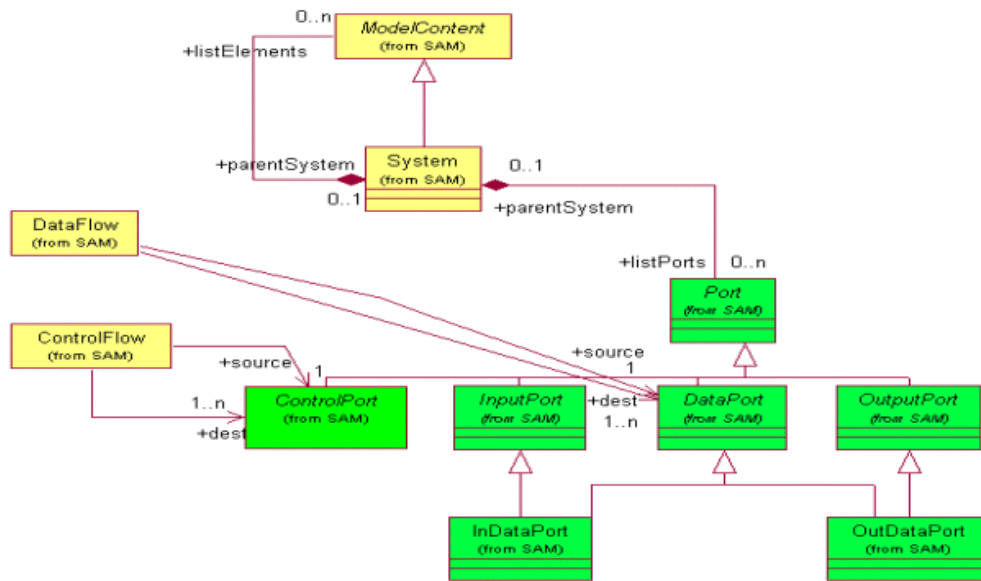
Figure 5: A simplified view of the SAM meta-model
