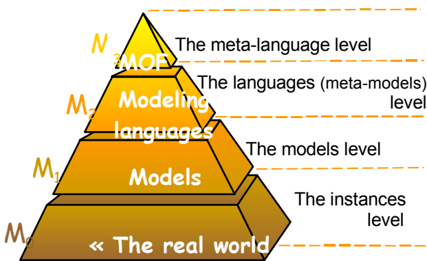
Figure1: The four-layer meta-model architecture.
